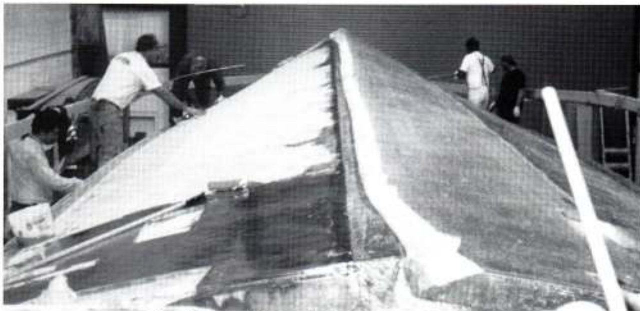
Sheathing a 65' Sportfish at Weaver Boatworks
